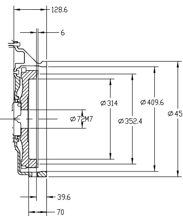
SECTION X-X
